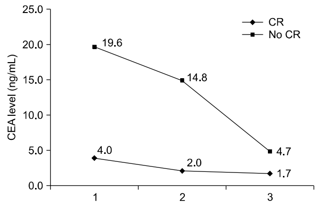
Fig. 1. Plot of CEA levels over time according to the response to chemoradiation.
